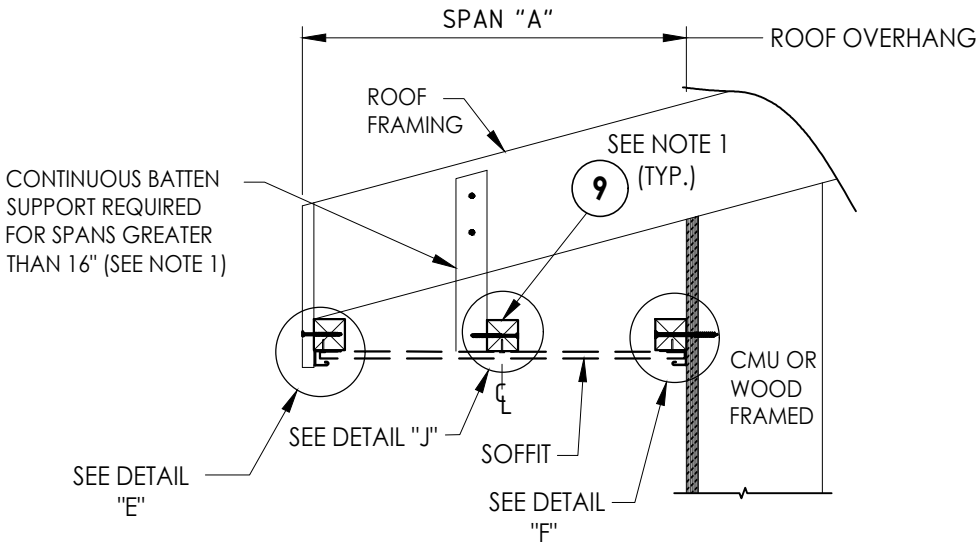
SIDE VIEW - DOUBLE SPAN w/ J-CHANNELS
