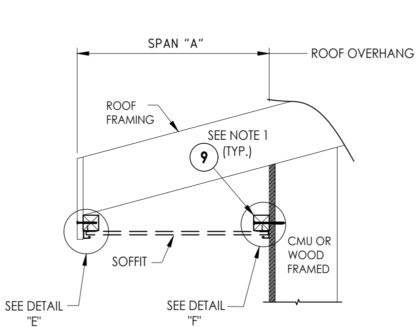
SIDE VIEW - SINGLE SPAN w/ J-CHANNELS
